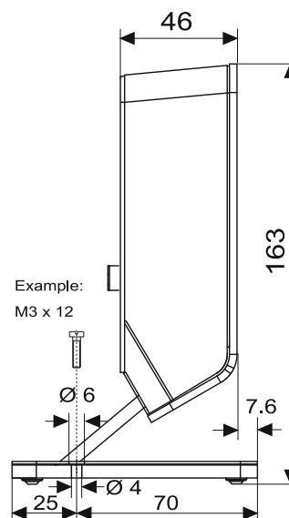
2 | Side view (dimensions in mm)
